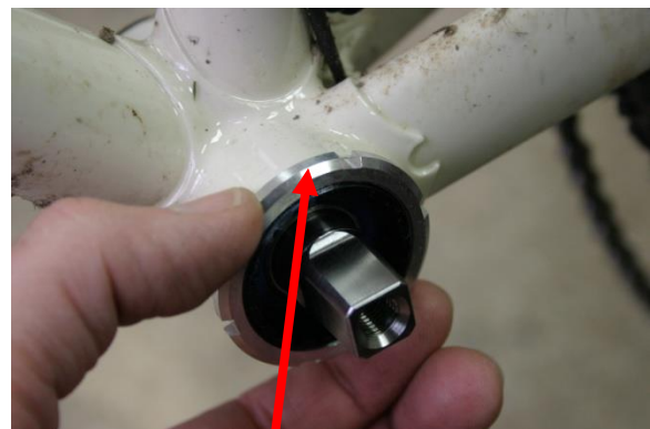
Fig.8 Beveled edge faces outward.
